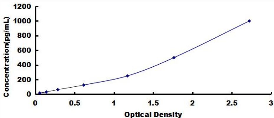
Typical Standard Curve of ELISA Assay for Human IFN \gamma .
